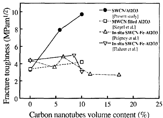
Figure 1. Fracture toughness versus carbon nanotube volume content in alumina based composites as reported in literature
