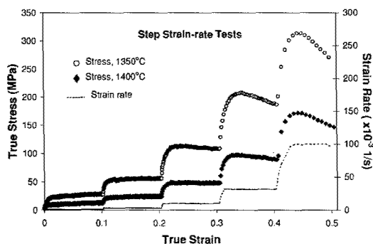
Figure 4. Typical stress-strain curves in the step strain-rate tests
