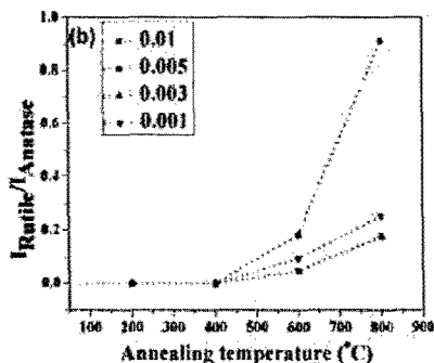
Figure 2(b) Variation of rutile:anatase phase contents as a function of calcination temperature
