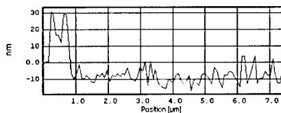
Figure 3: AFM image and section analysis of first Au layer of Au/Fe 3 O 4 /Au multilayer. Section analysis shows Au particles around 200 nm.
