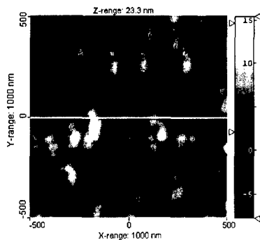
Figure 6: AFM image and section analysis of top layer of two-layer skutterudite film.
