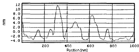
Figure 6: AFM image and section analysis of top layer of two-layer skutterudite film.
