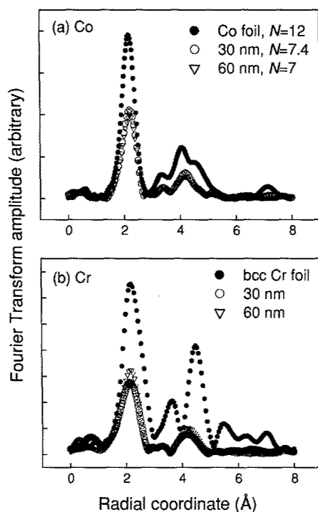
Figure 6. Fourier Transform Amplitude of (a) Co, and (b) Cr. N denotes the coordination number of the first shell
