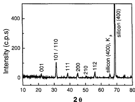
Figure 3. XRD of the \text{BaTiO}_3 nano-powder. The strong peak at 69^\circ was from the silicon wafer on which the powder was glued.
