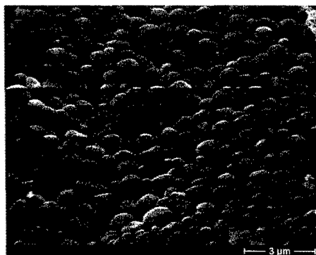
Figure 1. Microemulsion derived \text{BaTiO}_3 nano powder (dried at 450^\circ\text{C} )
