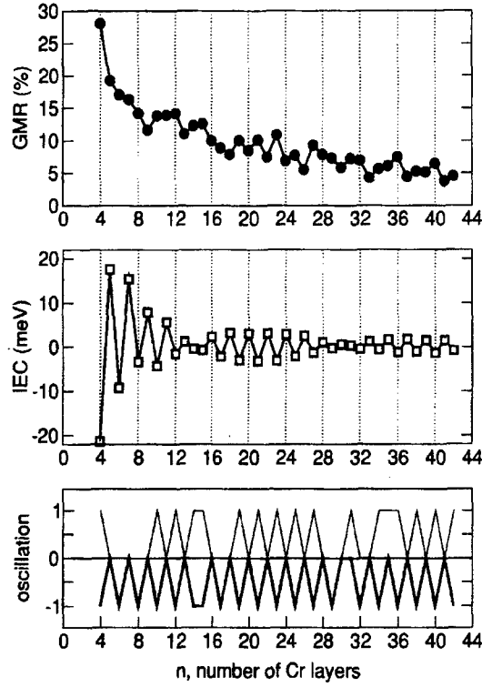
Figure 1. Top panel: The GMR of Fe/Cr/Fe trilayers depending on the thickness of the Cr Layer. Middle panel: The IEC for Fe/Cr/Fe as obtained from the band energy difference vs. the number of Cr layers. Bottom panel: Comparison of the oscillations of the GMR (thin lines) and the IEC (thick lines) of the above shown trilayers, for details see text.
