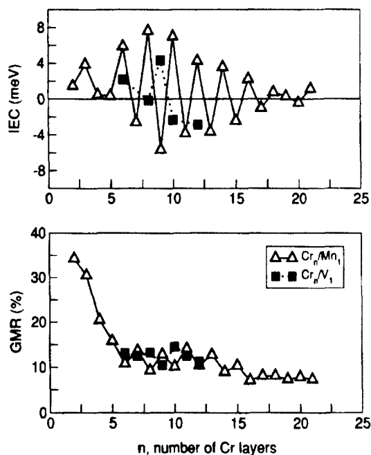
Figure 2. Top panel: The IEC of \text{Fe}/\text{Cr}_n/\text{T}_1/\text{Fe} multilayers vs. the number of Cr layers n . Two different types of impurity overlayers have been used: Mn (open triangles) and V (filled squares). Bottom panel: The GMR vs. the number of Cr layers for the above described systems.
