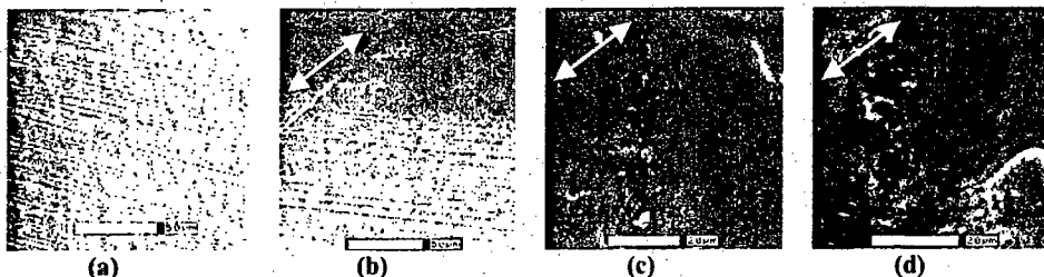
Figure 4. Representative ESEM micrographs of crosslinked UHMWPE surfaces obtained (a) before and after testing for (b) 27,000 (c) 26,200 and (d) 18,400 sliding cycles. (Sliding occurred against (b) smooth and (c), (d) rough Co-Cr counterfaces. Arrows denote direction of sliding.)
