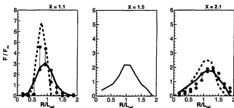
FIGURE 9. Comparison of radial variation of liquid axial mass flux at various axial locations, ---- P&W RANS with TAB model, — present LES with stochastic model, o — o experimental error bar.
