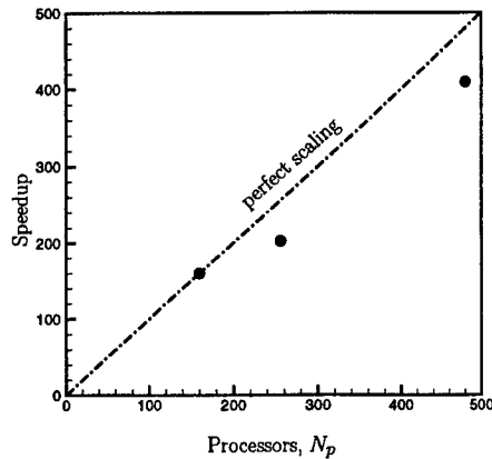
FIGURE 4. Scalability of the new CDP- \alpha code on Frost (with hypr AMG solver for pressure). Problem is the cold flow LES of the full combustor geometry with 35 M cv's. Scaling is reported relative to the 160 processor case, which was the smallest number of Frost processors that could run this problem.
