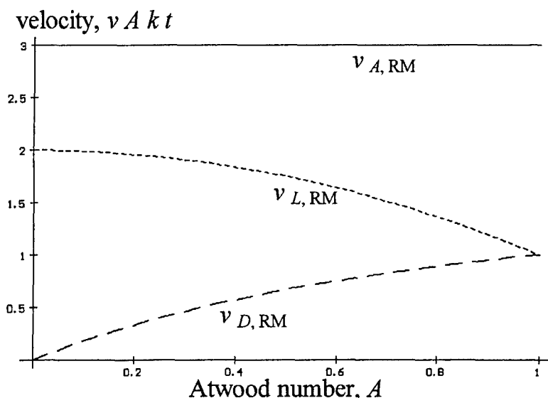
FIGURE 3. Dependence of the bubble velocity v on the Atwood number A for 3D highly symmetric flows in the Richtmyer-Meshkov instability; k is the wavevector, t is time, v_{L, RM} = (2 - A^2)/Akt is the Layzer-type solution, v_{D, RM} = 2/(1 + A)kt is given by the drag models, v_{A, RM} = 3/Akt is given by the RM multiple harmonic non-local solution.
