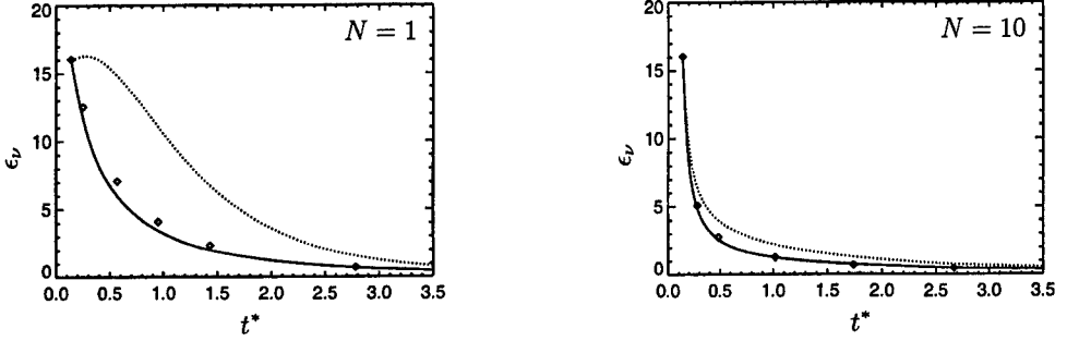
FIGURE 5. Resolved viscous dissipation rate \epsilon_v for the cases N = 1 (left) and N = 10 (right). In each plot, the solid line represents the LES, the diamonds represent the filtered DNS and the dotted line represents the unresolved DNS.
