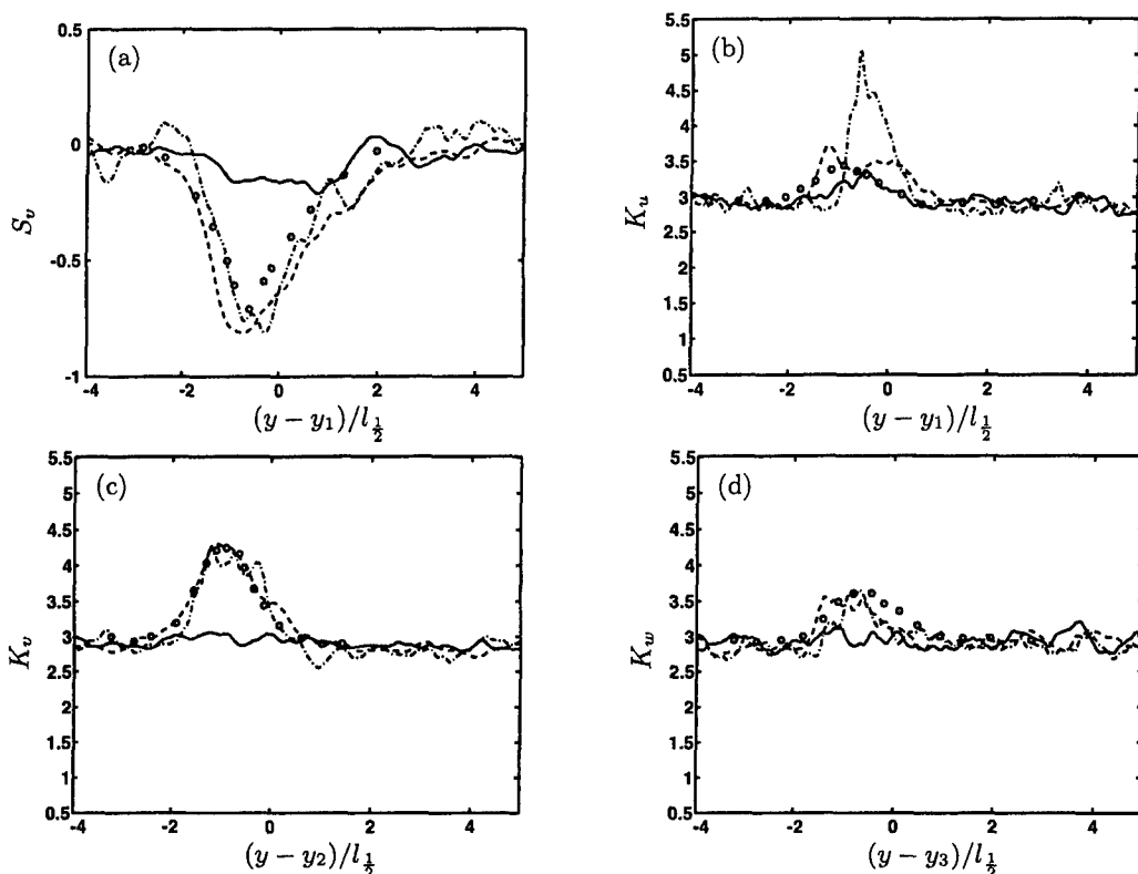
FIGURE 5. (a) Skewness of v ; (b) Kurtosis of u ; (c) Kurtosis of v ; (d) Kurtosis of w ; — : t^* = 0 ; ---- : t^* = 0.56 ; -.- : t^* = 1.51 ; o: experimental data from Veeravalli & Warhaft (1989). At t^* = 0 the numerical curves are close to their Gaussian value since the penetration mechanism described in the text has not occurred yet.
