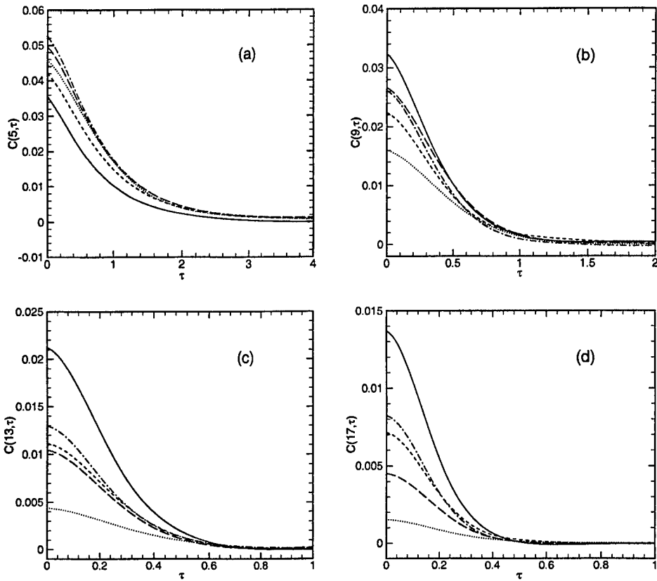
FIGURE 4. Time correlation C(k, \tau) vs time lag \tau with starting time t = 1.5 for (a) k = 5 , (b) k = 9 , (c) k = 13 , (d) k = 17 . — DNS; ---- dynamic Smagorinsky model; —·— multiscale LES; ..... Smagorinsky model; - - - spectral eddy viscosity model.
