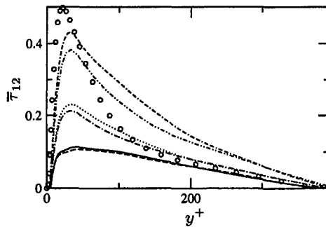
FIGURE 5. Modeled shear stress, \bar{\tau}_{12} , using different turbulence-closure models. \circ : filtered DNS, — : DSM (64,49,48), ---- : DSM (128,97,96), — · — : DMM (64,49,48), ..... : DMM (128,97,96), — — — : DRM (N=5) (64,49,48), and · — · : DRM (N=5) (128,97,96).
