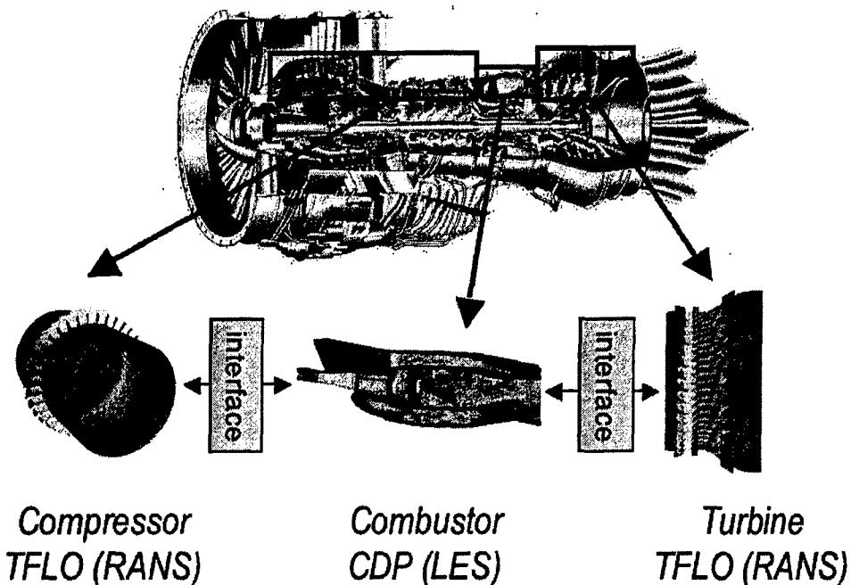
FIGURE 1. Decomposition of gas turbine engine. LES of combustor (Mahesh et al. 2001; Constantinescu et al. 2003), RANS of turbine section (Davis et al. 2002)
