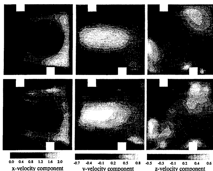
FIGURE 7. Comparison between simulations (top) and experiments (bottom) in region 3 (see Fig. 2): vertical plane corresponding to a cross-section before the U-bend.
