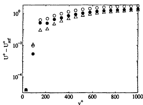
FIGURE 4. Error in the mean velocity profiles with respect to their references. \circ , case S1; \bullet , case S2; \triangle , case R1.
