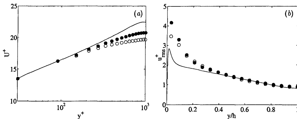
FIGURE 2. Profiles of (a) the mean velocities and (b) the streamwise velocity fluctuations for a smooth-walled channel at Re_\tau \approx 1000 , using different cost functions. \circ , case S1; \bullet , case S2; —, direct simulation (del Álamo et al. 2003).
