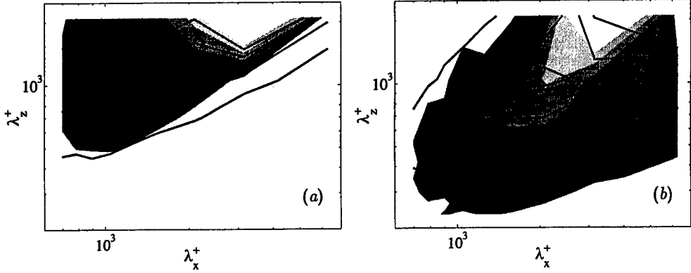
FIGURE 6. Two-dimensional premultiplied spectra of the stresses at the wall as functions of the streamwise and spanwise wavelengths. (a) E_{xy} , (b) E_{zx} . Shaded contours are from the S1 case and lines are from R1. Each spectrum is normalized with its maximum.
