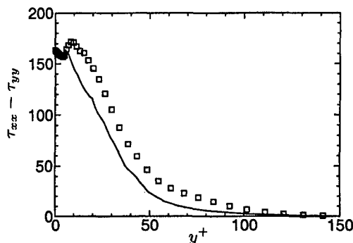
FIGURE 1. Left : Normal stress profiles of the viscoelastic simulation L100W120MC, \square , compared to the Brownian dynamic simulation, —.
