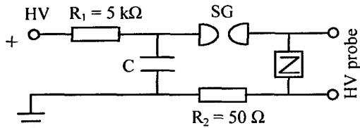
Fig. 1. Experimental set-up
