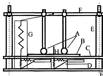
Figure 1 Experimental setup
