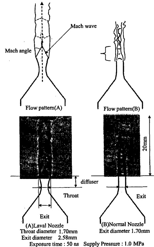
Fig.2 Shape of nozzles and visualization of gas by shadowgraph technique.
