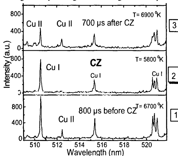
Fig. 3 Emission spectra around CZ
