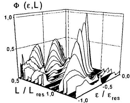
Figure 2: Amplitude of the distribution function \Phi(\varepsilon) calculated for different values of spatial period L .
