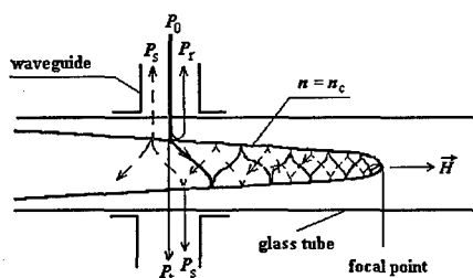
Fig. 1. Scheme of excitation and propagation of the EPW. P_0 , P_1 , P_s , P_r are incident, transient, scattered and reflected power correspondingly.
