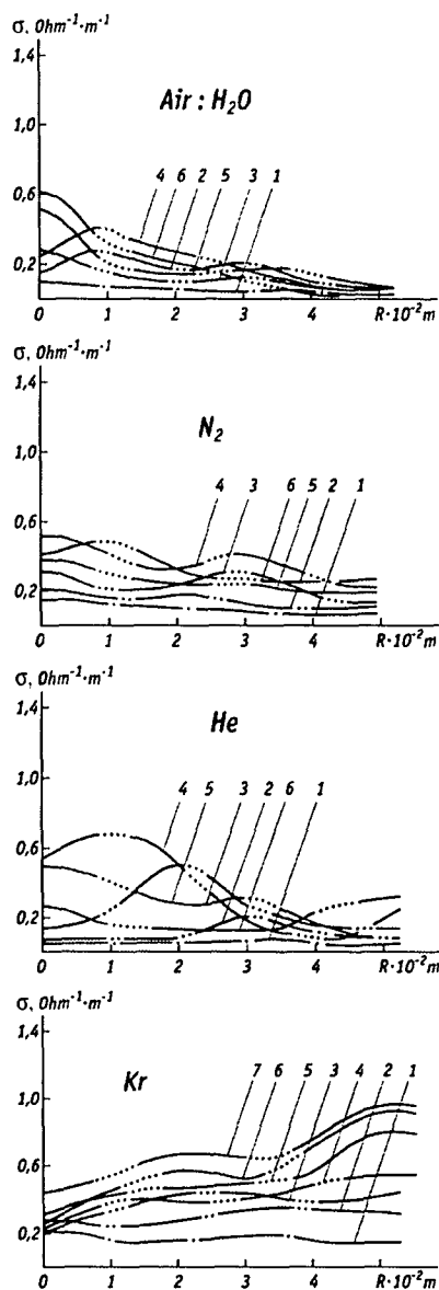
Fig.1. Radial conductivity profile of plasma channel created by REB in gases (at pressure P = 300 \text{ Tor.} ). The time elapsed from the beginning of a pulse: 1- 10 ns., 2- 20 ns., 3 - 30 ns., 4 - 40 ns., 5- 50 ns., 6- 60 ns., 7- 70 ns., 8- 80 ns.
