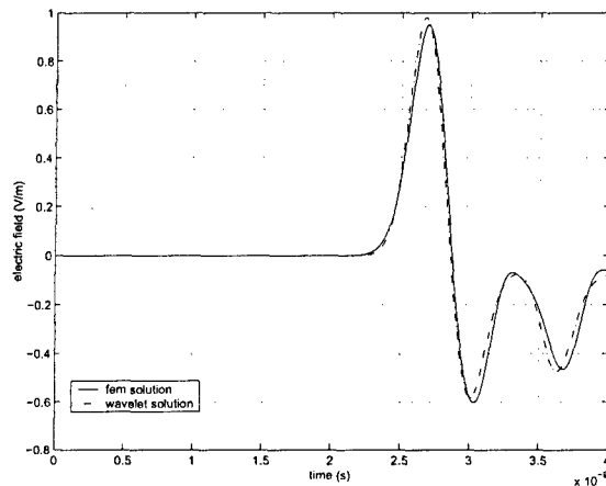
Fig. 8. Electric field evaluated at point P \equiv (0, -0.2)
