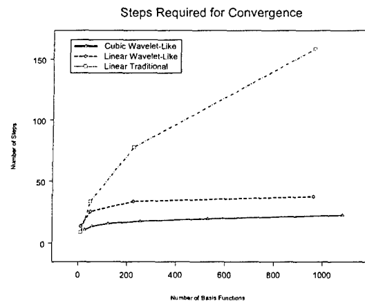
Fig. 22. Steps required for convergence.
