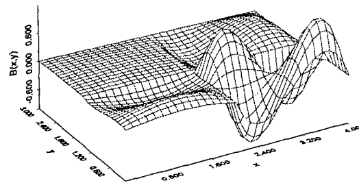
Fig. 15. Cubic wavelet-like basis function obtained from a 2 nd level x and 2 nd level y function.
