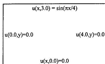
Fig. 16. Problem domain.
