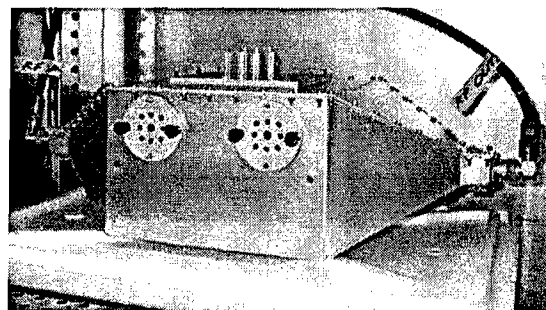
Figure 2. TEM Cell placed in the incubator (with ventilation holes shown).
