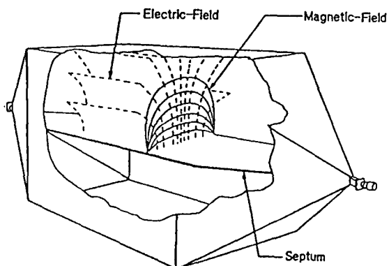
Figure 1. The electric and magnetic fields within a TEM cell, with a plane wave type structure at the midpoint of the top half.
