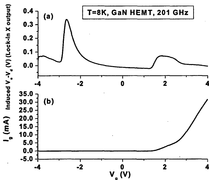
Fig. 3. (a) The GaN HEMT detector response to 201 GHz radiation at T=8\text{ K} and (b) Gate current versus gate voltage for the positive (forward) gate bias at 8 K.
