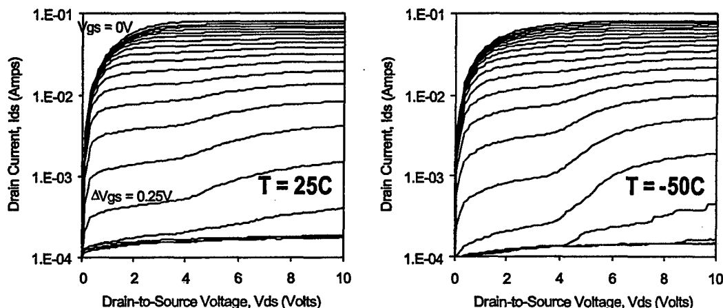
Figure 2 a) Output characteristics of an 80 \mu m wide AlGa N /Ga N HEMT at room temperature. The logarithmic scale is chosen to highlight the increase in the output conductance at lower drain currents. V_{gs} is stepped from 0 to -5V. b) Output characteristics of the device from Fig. 1 at -50C. The impact ionization rates increase at lower temperatures and the enhancement in the output conductance is more pronounced.
