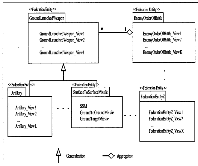
Figure 5. Federation Interoperability Object Model (FIOM) Representation
