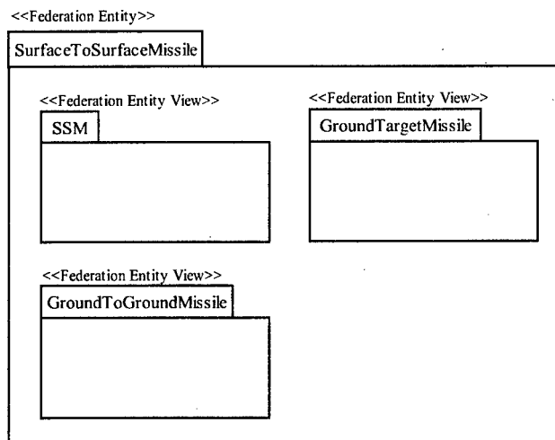
Figure 4. Defining Federation Entity (FE) and Federation Entity Views (FEVs) for Real-World Entity
