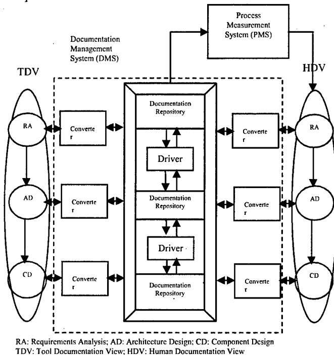
Figure 1. Documentation Driven Agile Software Development
