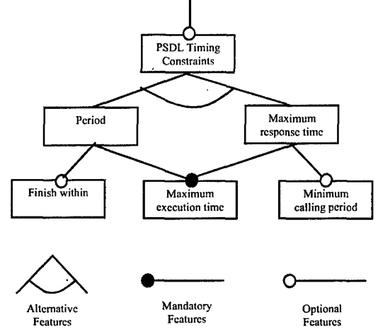
Figure 3. Feature Model of the PSDL Timing Constraints of CAPS
