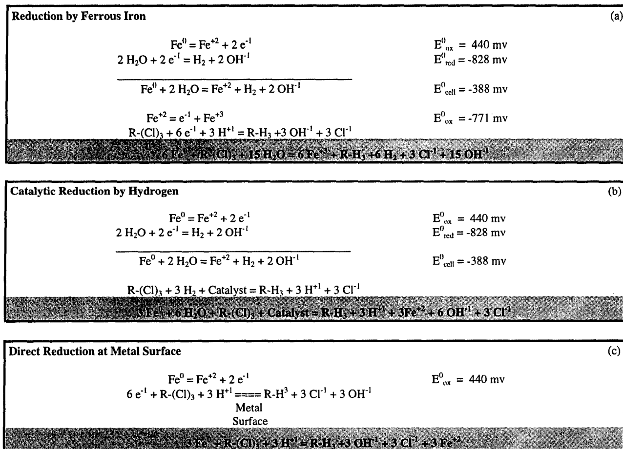
Figure 3. Suggested Chemical Mechanisms for the Reductive Dechlorination of Dissolved-Phase CAHs in the Presence of Iron. (Stoichiometrically Balanced Equations for Degradation of TCE by Each Mechanism are Contained in the Shaded Box.)
