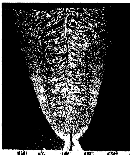
a) Hybrid laser weld
