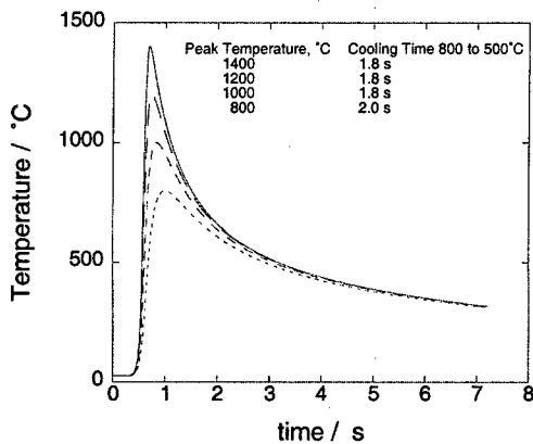
(a) autogenous laser weld
