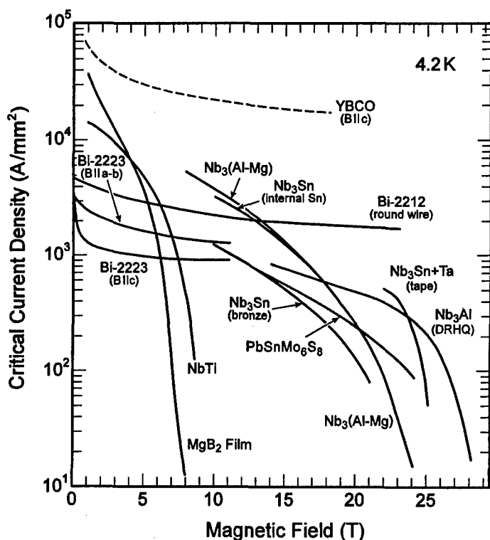
Figure 2. Critical current density as a function of magnetic field for a number of high-field superconductors at liquid-helium temperature (from a compilation by Lee 8 ). Data are referenced to the superconducting-material area alone, as opposed to the entire cross section of the wire, which contains structural and stabilizer materials needed for the practical use of superconductors.
