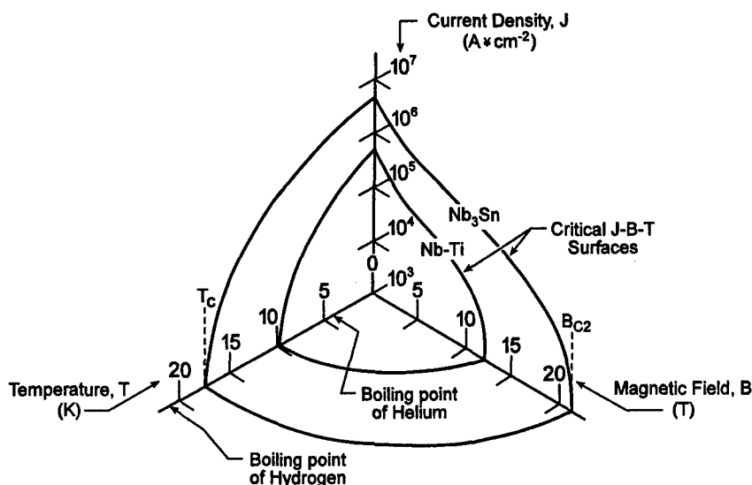
Figure 1. Critical-current density J_c of two commercial low-temperature superconductors as a function of magnetic field B and temperature T . In the region between the origin and the critical J - B - T surface, the material is superconducting; above the surface the superconductor reverts to the normal resistive state.
