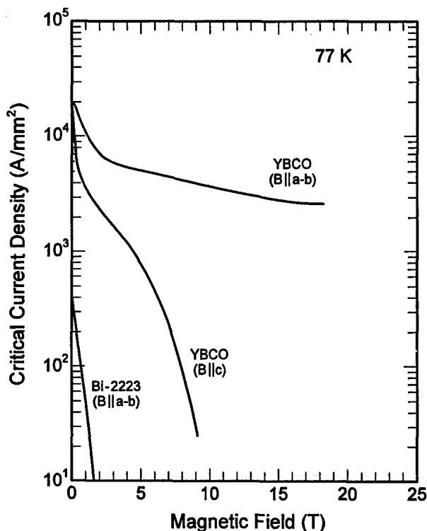
Figure 3. Critical-current density as a function of magnetic field for high- T_c superconductors at liquid-nitrogen temperature (from a compilation by Lee 8 ). The critical-current density J_c is referenced to the superconductor area alone.
