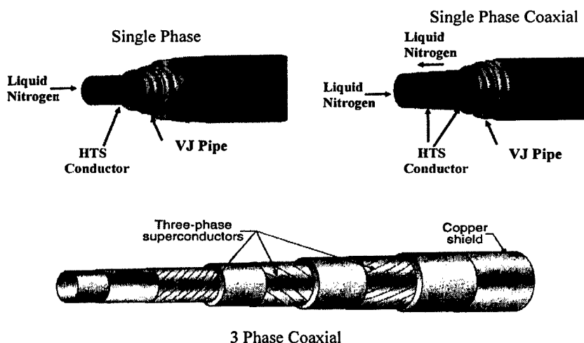
Figure 5. Three types of HTS power cables being developed and tested: single phase, single-phase coaxial, and 3-phase coaxial (or triaxial). All are cooled by flowing liquid nitrogen and thermally insulated with vacuum-jacketed (VJ) pipe (from Southwire).
