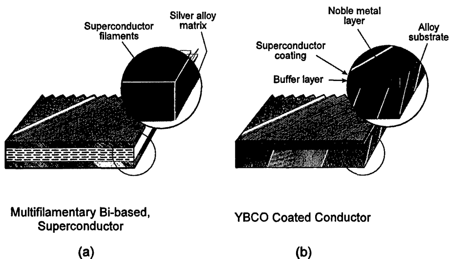
Figure 4. Cross-sectional view of practical high- T_c superconducting composites: (a) multifilamentary (\text{Bi,Pb})_2\text{Sr}_2\text{Ca}_2\text{Cu}_3\text{O}_{10-x} (Bi-2223) silver-alloy-sheathed high- T_c superconductor tape; (b) coated thick-film \text{YBa}_2\text{Cu}_3\text{O}_7 (YBCO) superconductor tape (from American Superconductor).
