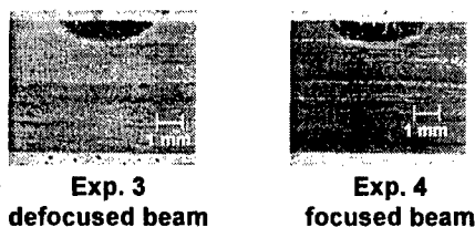
Figure 4 – Micrographs of results produced by the pre-heating pass of experiments 3 and 4.
