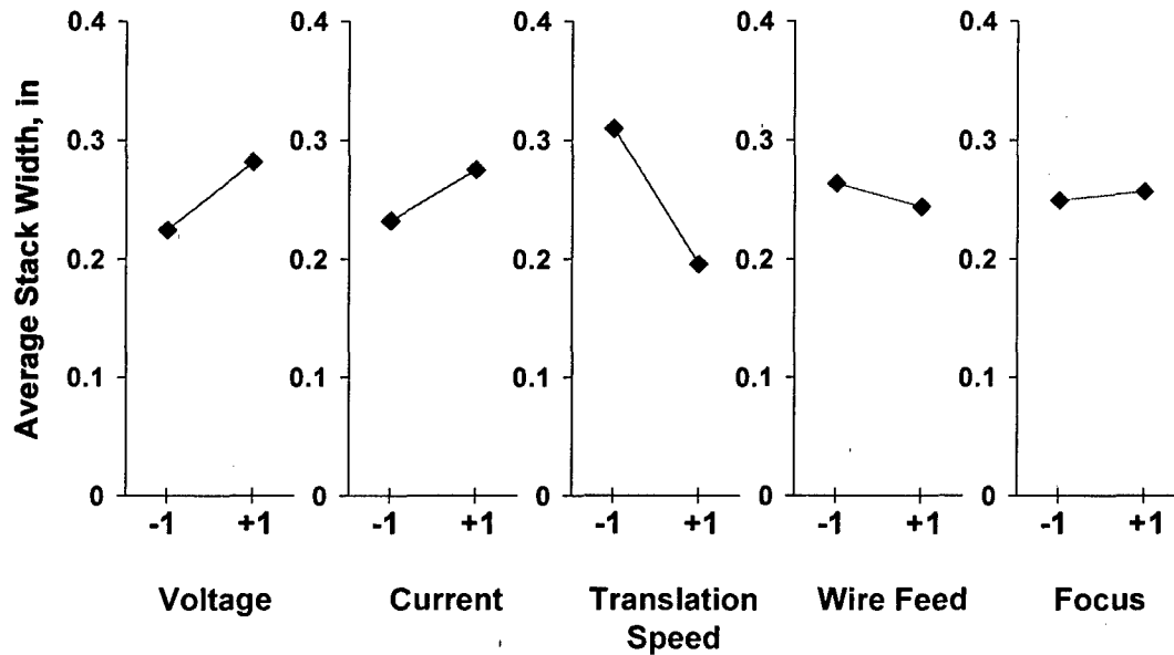
Figure 8. Marginal mean plots for average stack widths
