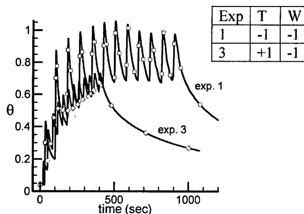
Figure 2. Normalized temperature history on the back side of the plate during the multi-bead stacks produced by experiments 1 and 3
