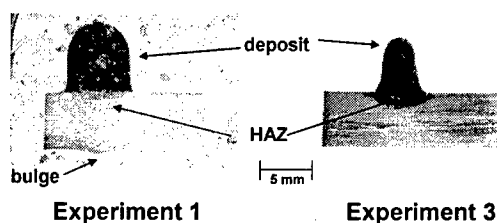
Figure 1. Micrographs of multi-bead stacks produced by experiments 1 and 3.
