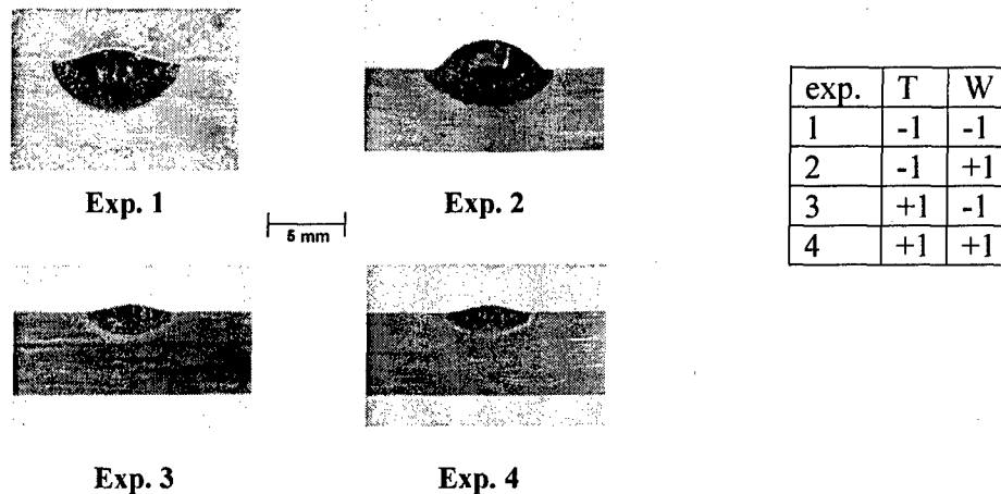
Figure 7. Micrographs of single bead passes produced by experiments 1 through 4.
