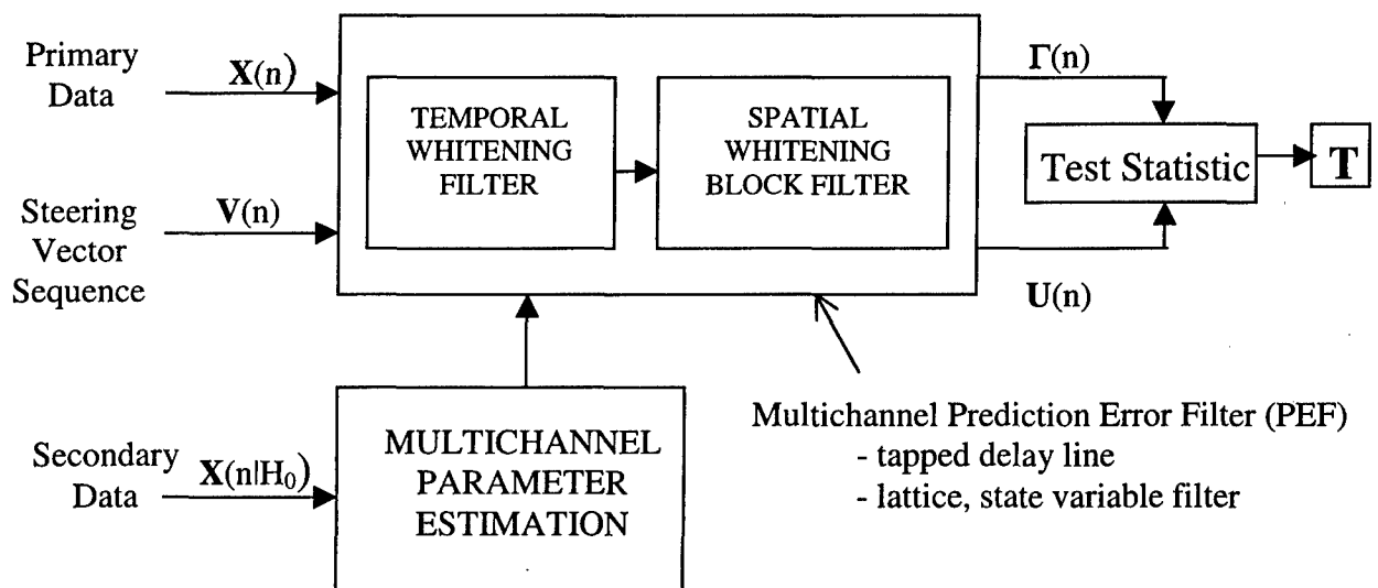
Figure 4: Parametric STAP
