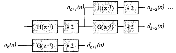
Figure 1 - Wavelet Decomposition
