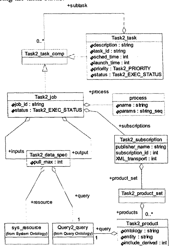
Figure 6. Task Ontology
