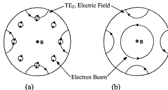
Figure 1. Schematic of electrons interacting with a TE_{21} mode in a circular waveguide for (a) a non-axis-encircling beam and (b) an axis-encircling beam.
