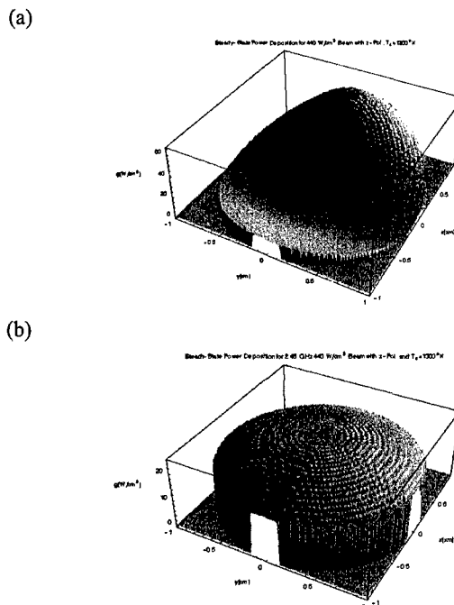
Figure 4. Steady-state power deposition for a 2.45 GHz, z-polarized beam in a rotating alumina cylinder. (a) Instantaneous deposition, (b) averaged deposition.
