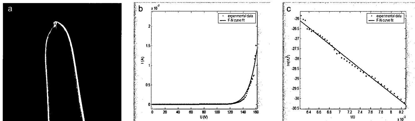
Figure 1. (a) Scanning electron microscopy (SEM) image of a multi-walled carbon nanotube (MWNT) attached to an electrochemically etched nickel wire. (b) Current-voltage field emission data of the MWNT in (a), with the Fowler-Nordheim equation curve fit. (c) Fowler-Nordheim plot of the same data.
