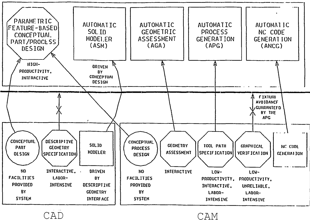
Figure 7. Illustration of Seamless DTM Systems.
