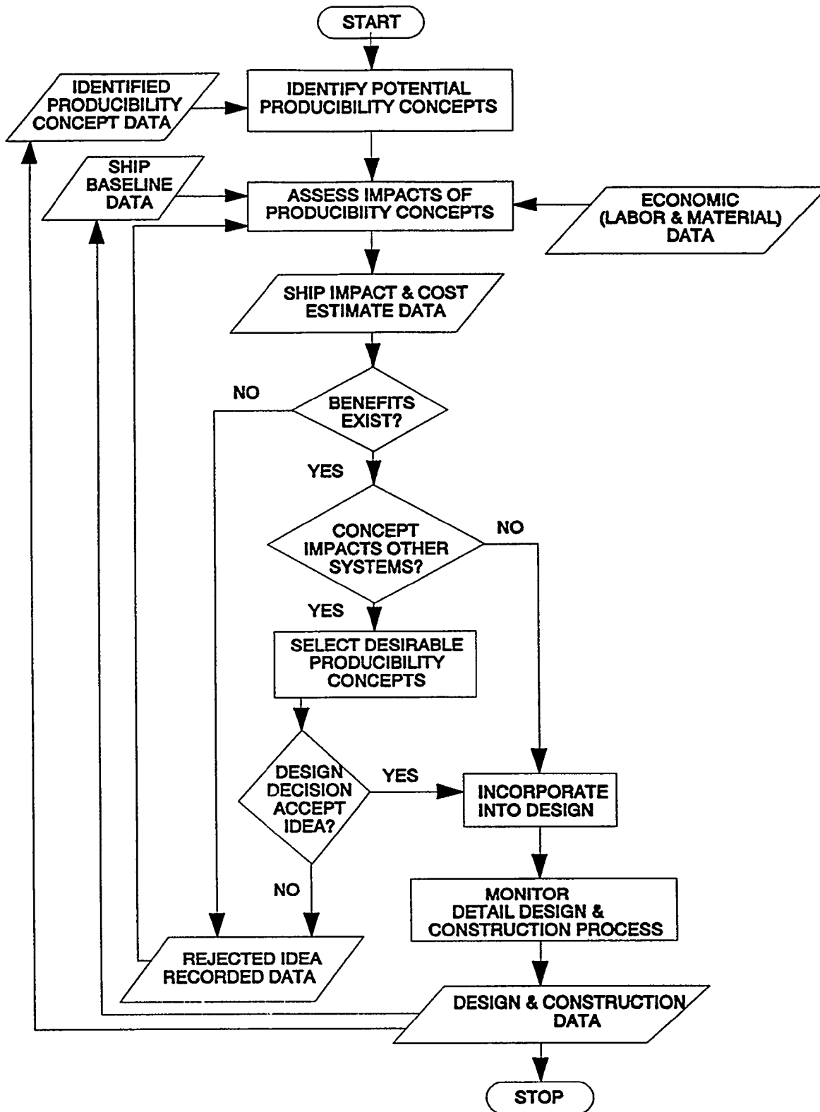
Figure 4 Framework for Producibility Design Decisions
