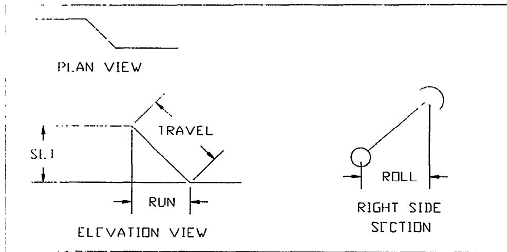
Figure 2. Typical Pipe Center Line Sketch
