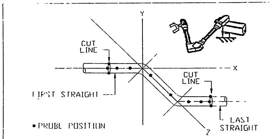
Figure 6. Typical Pipe Configuration Measured by PCMM
