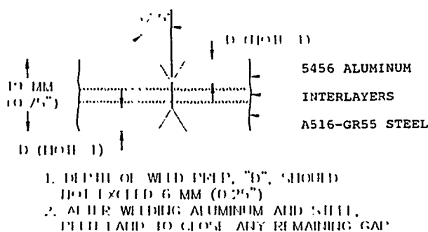
FIGURE 1: Design of butt joints between ends of transition joint strips.
