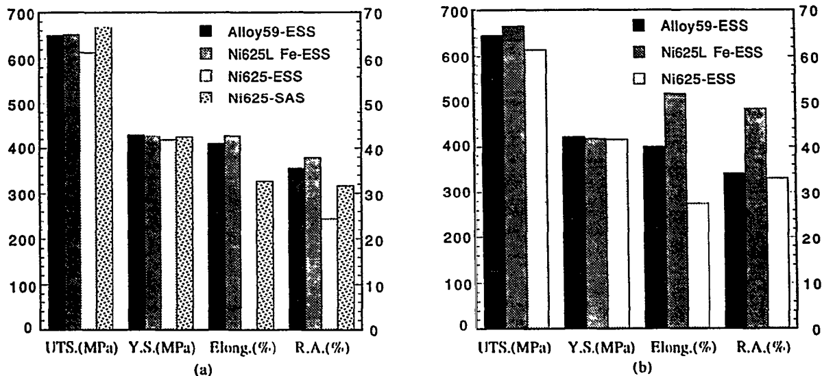
FIGURE 5. Tensile Properties of 25 mm (1 inch) Thick Cladding Deposited in Five Layers with Ni Alloy Strips on MIL-S-23294, Class 1 Steel Using ESS; (a) As-welded and (b) Post-weld Stress Relieved.
