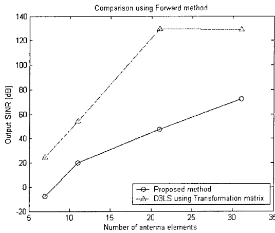
Fig. 5(a). Comparison of the output SINR between the proposed method and a more accurate compensation for mutual coupling using the Forward processor.
