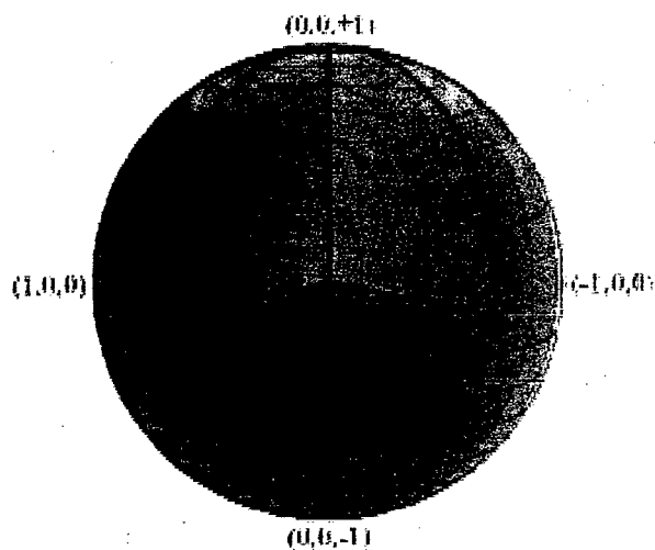
Figure 3. The colorized Poincaré sphere of unit radius. On the surface of the sphere P = 1 , at the center P = 0 , inside the sphere P < 1 .
