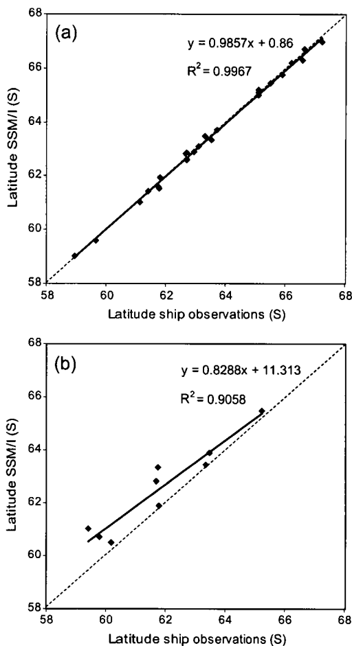
Fig. 3. Comparison of ice edge position from satellite data and ship observations: (a) winter (March–October) and (b) spring–summer (November–December). The dashed line in both is the one-to-one line (Worby & Comiso 2001).
