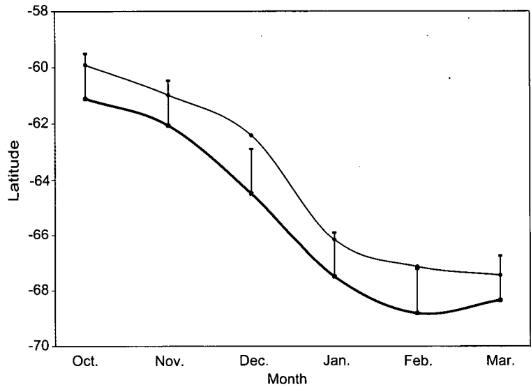
Fig. 4. Sea ice extent plotted as latitude against month, October–March. The lower curve shows the values from modern satellite data (1979–1998). The upper curve represents data from digitized maps in Mackintosh (1972) for 1925–1952. The topside bar on the satellite data is an estimate of 1.6° latitude northward, given the differences in ship observations and ice extent for the summer period.
