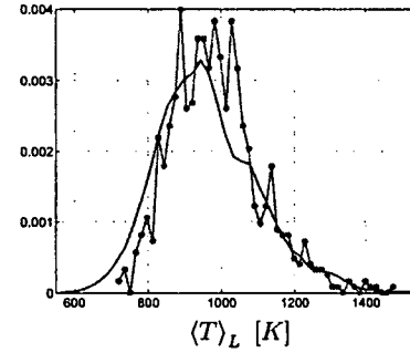
FIGURE 4: PDFs of the resolved (a) mixture fraction, and (b) temperature at the radial location r = 5.05 \text{ mm} compared to the experiment. (top-to-bottom rows) x/D_B = 0.9 , and 1.3 . — FDF, —●— Experiment.
