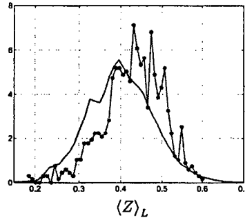
FIGURE 4: PDFs of the resolved (a) mixture fraction, and (b) temperature at the radial location r = 5.05 \text{ mm} compared to the experiment. (top-to-bottom rows) x/D_B = 0.9 , and 1.3 . — FDF, —●— Experiment.
