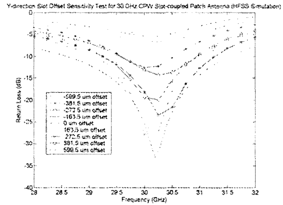
Fig. 13. HFSS-simulated S_{11} for wafer-scale patch antenna y-direction slot alignment sensitivity test.
